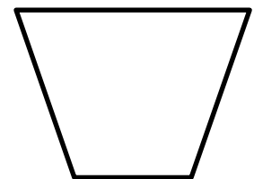
Trapez
