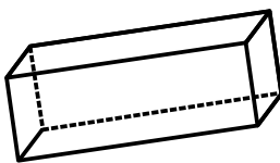
Quader
