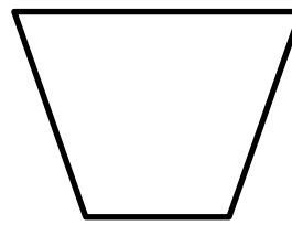
Trapez
