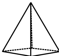
Pyramide
