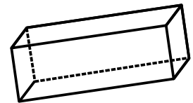
Quader
